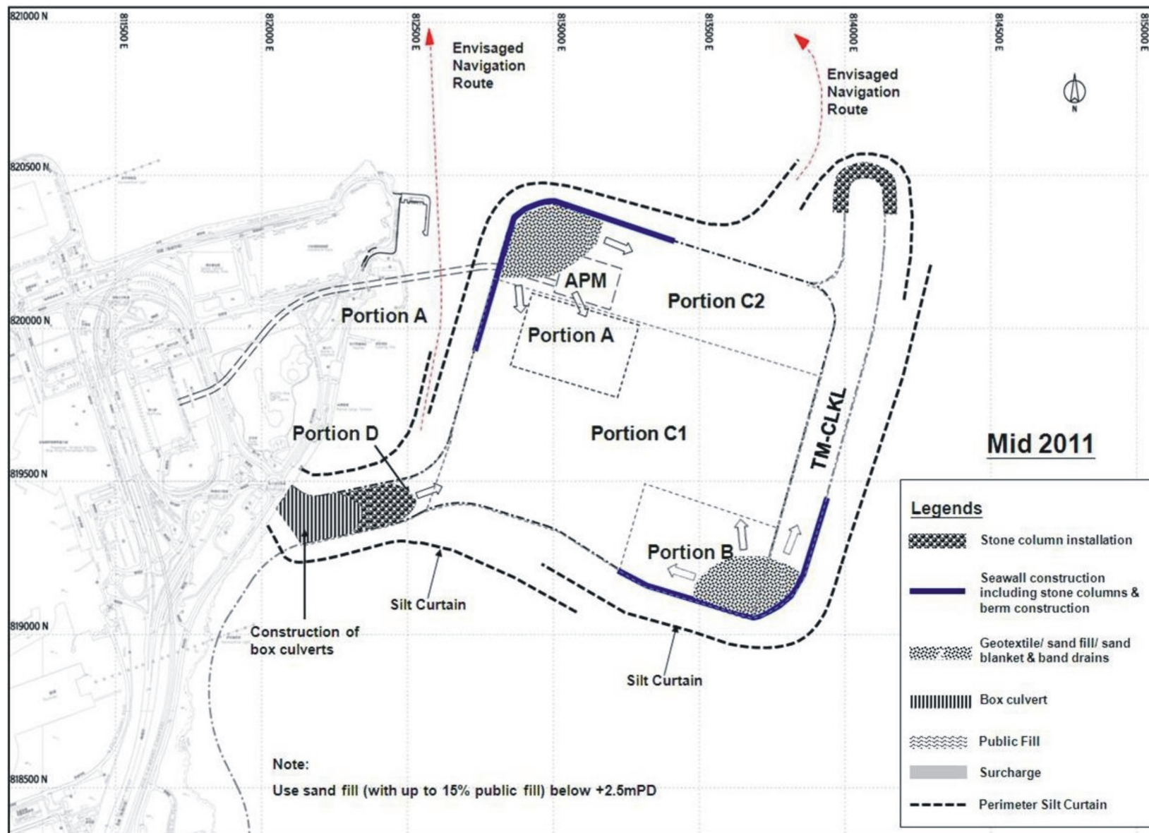
Figure 13 - Outline of Construction Sequence (Sheet 2 of 10) 圖 13 - 施工程序大綱(表10之2)
